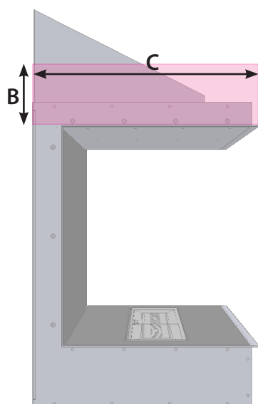
NON-Combustible Facing Dimensions (Left Side)
