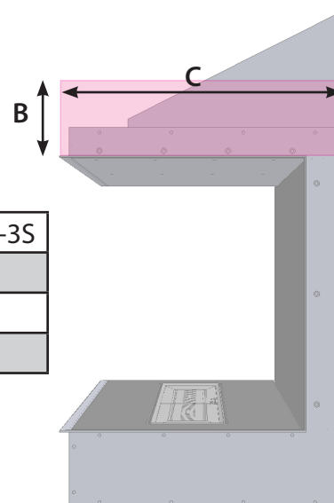
NON-Combustible Facing Dimensions (Right Side)
