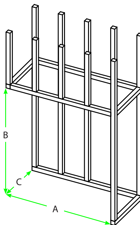
Rough Opening for HVF-42-LC, HVF-60-LC and HVF-72-LC
