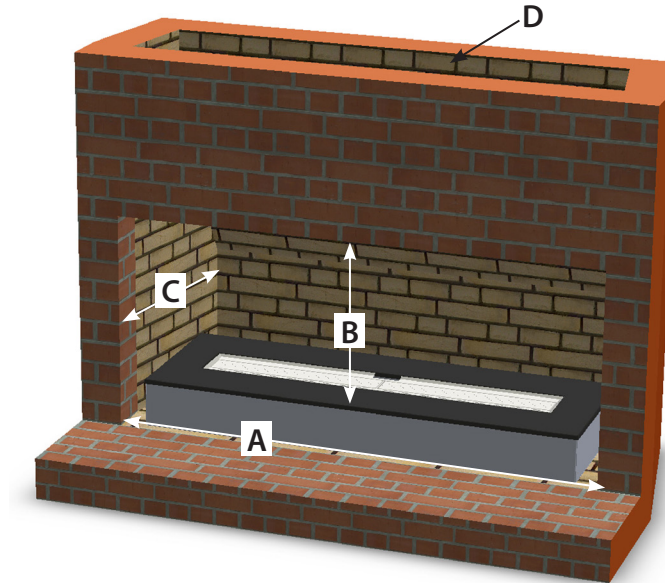
Minimum Fireplace Dimensions Required by Model
