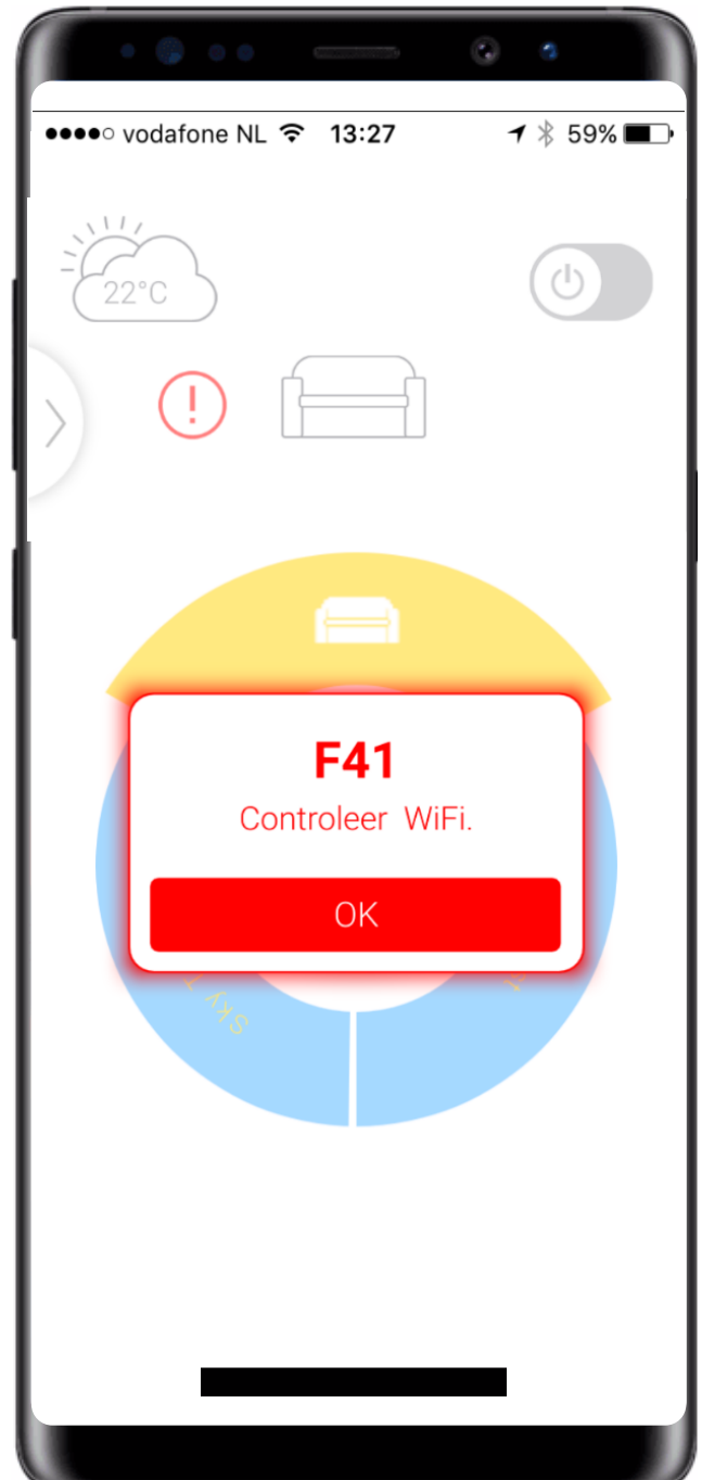
Figure 104: Application screen
