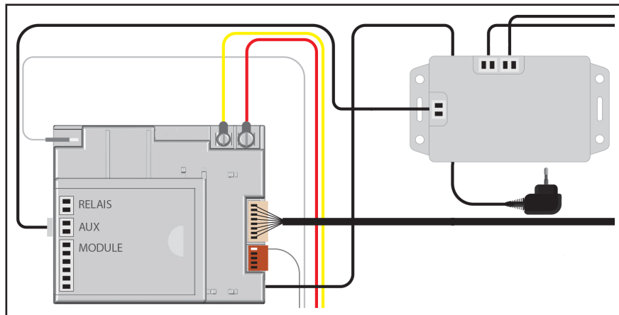
Figure 5: AC Adapter Connection
