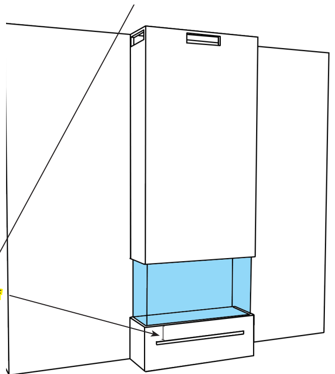
Figure 48: Trisore 140 GSB with Wall Outlets
